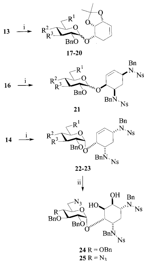
Scheme 3. Reagents and conditions: i. Donor (1.2 equiv.), NIS (1.2 equiv.), \text{TfOH} (0.1 equiv.). ii. \text{K}_2\text{OsO}_4 \cdot 2\text{H}_2\text{O} (0.5 mol %), NMO (2.2 equiv.), acetone/ \text{H}_2\text{O} (2.5:1, v/v) 24 : 99%, 25 : 88%
