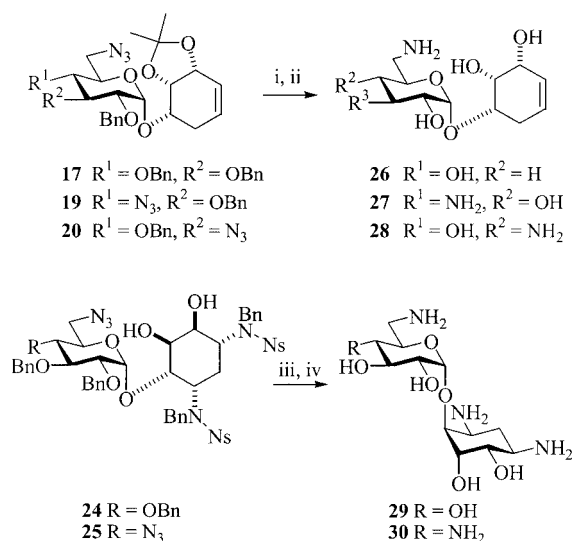
Scheme 4. Reagents and conditions: i. HOAc/H 2 O 8:2, reflux, 80–88% ii. Na (s), NH 3 (l), THF, −40 °C, 52–67%. iii. PhSH, dipea, DMF; 48–53% iv. H 2 /Pd-C, 0.1 M HCl; H 2 O/EtOH, 1:1; 29 : 68% 30 : 42%
