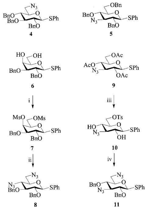
Scheme 1. Reagents and conditions: i. \text{MsCl} (2.5 equiv.), pyridine, 90%. ii. \text{NaN}_3 (4 equiv.), DMF, 80 °C, 78%. iii. a. \text{KOtBu} (0.1 equiv.), \text{MeOH} . b. \text{TsCl} (1.1 equiv.), pyridine, 67%. iv. a. \text{NaN}_3 (3.0 equiv.), DMF, 80 °C. b. \text{NaH} (2.1 equiv.), \text{BnBr} (2.1 equiv.), DMF, 93%
