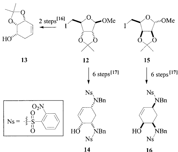
Scheme 2. Synthesis of acceptors
