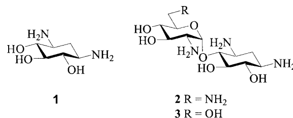
Figure 1. 2-Deoxystreptamine ( 1 ), neamine ( 2 ) and paromamine ( 3 )
